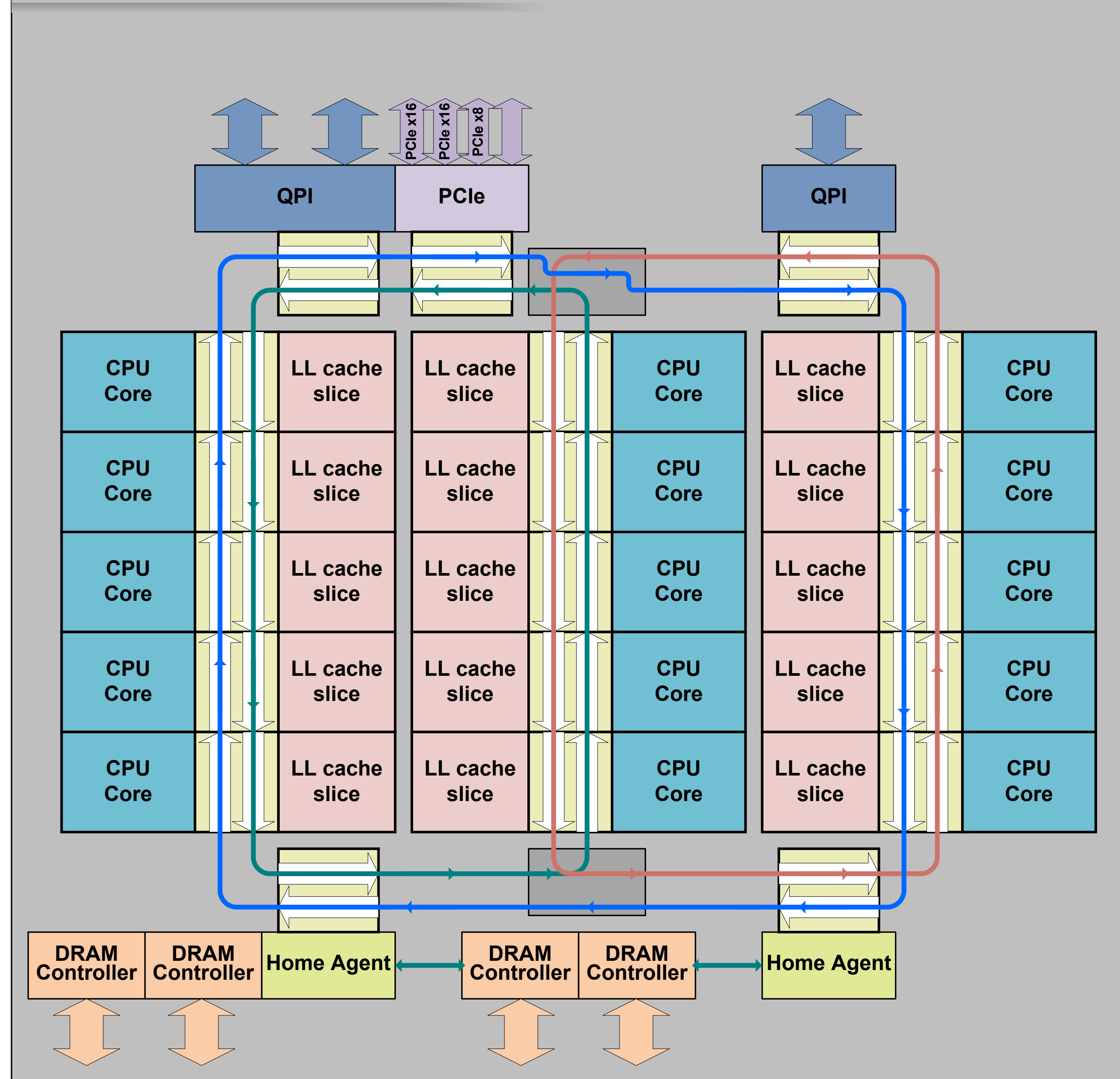
IvyTown 15Cores Ring Bus VRing0
