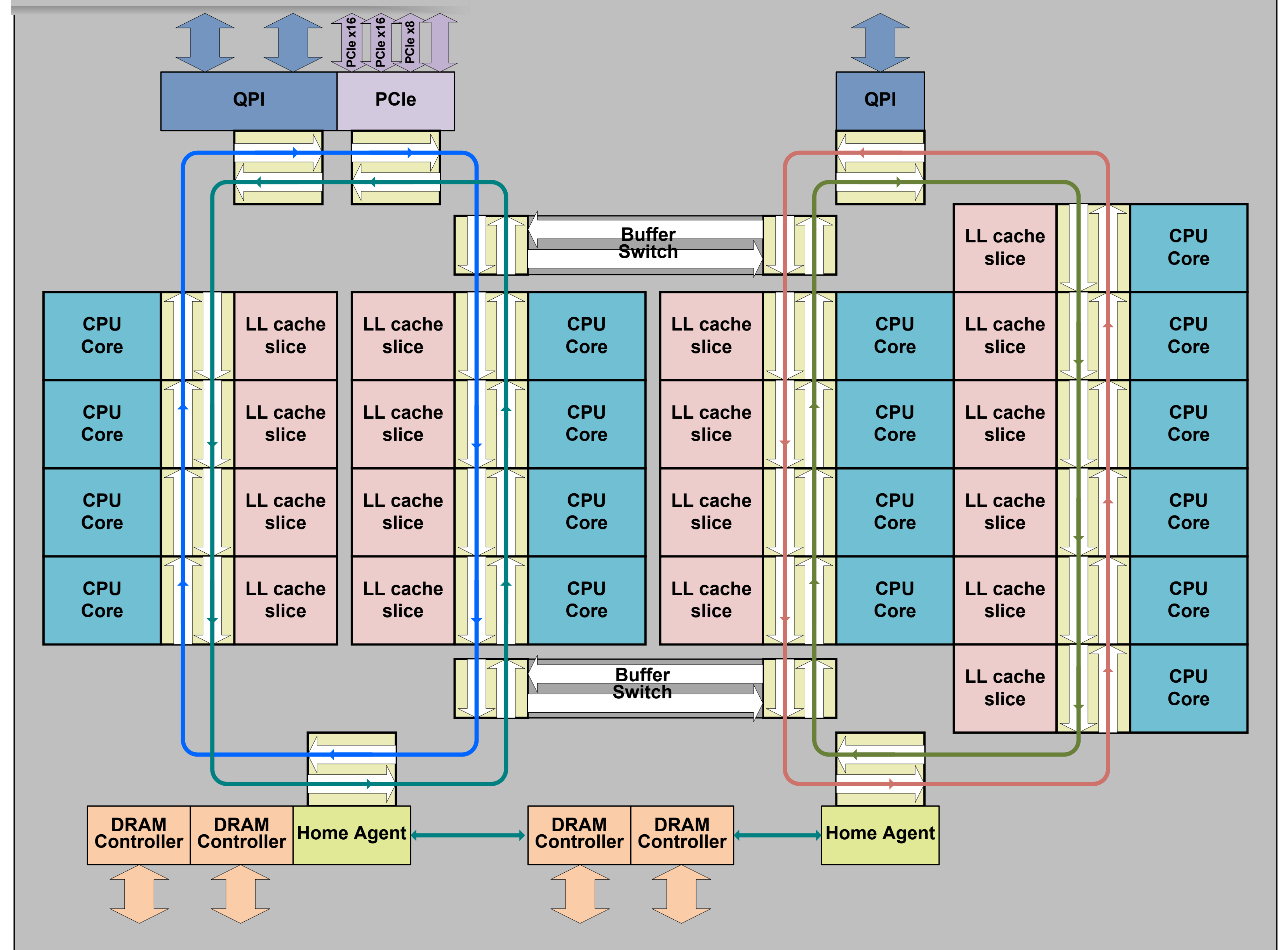
Haswell-E 18Cores Ring Bus
