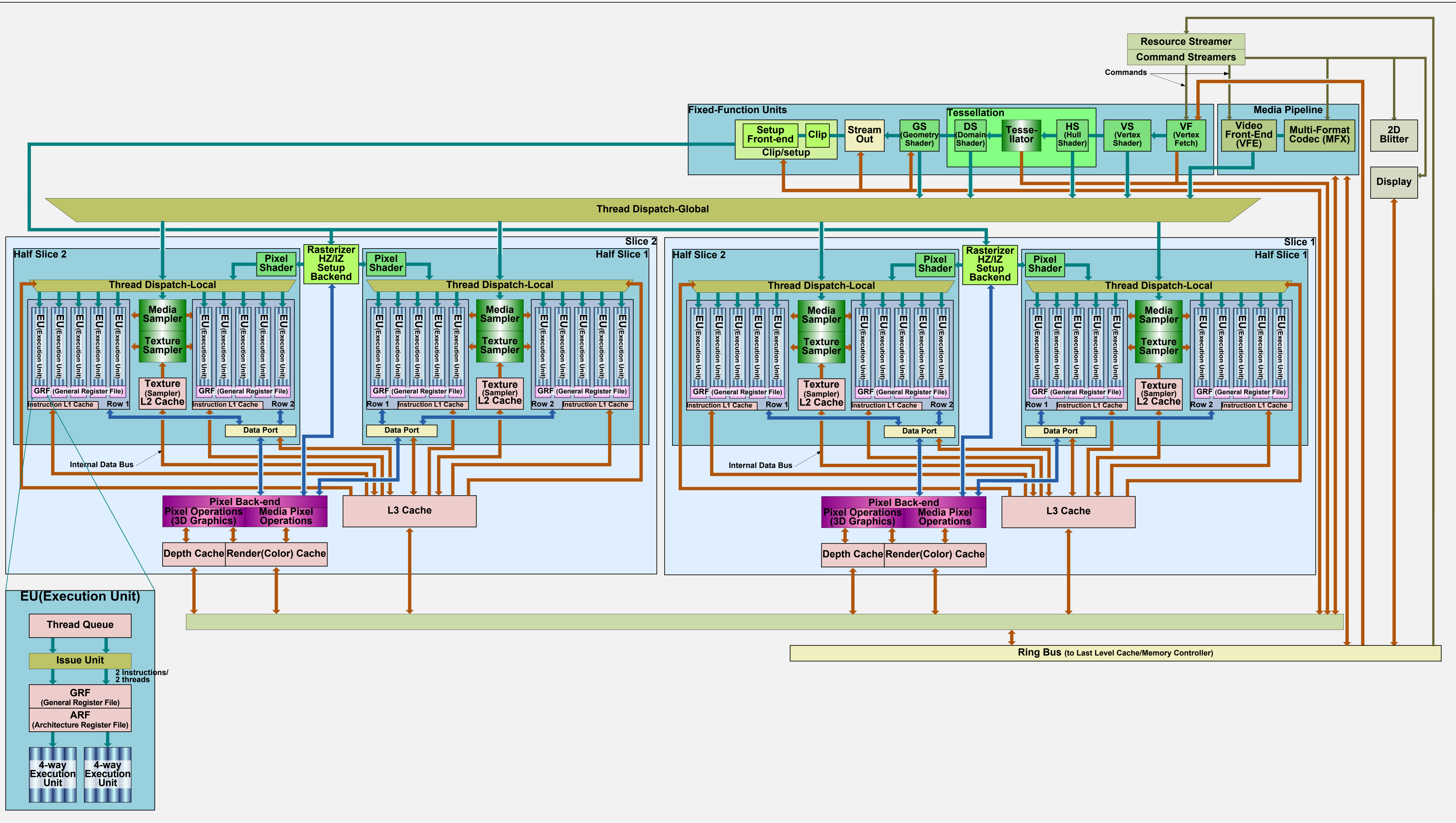
Intel Haswell Graphics Core Diagram (estimated)
