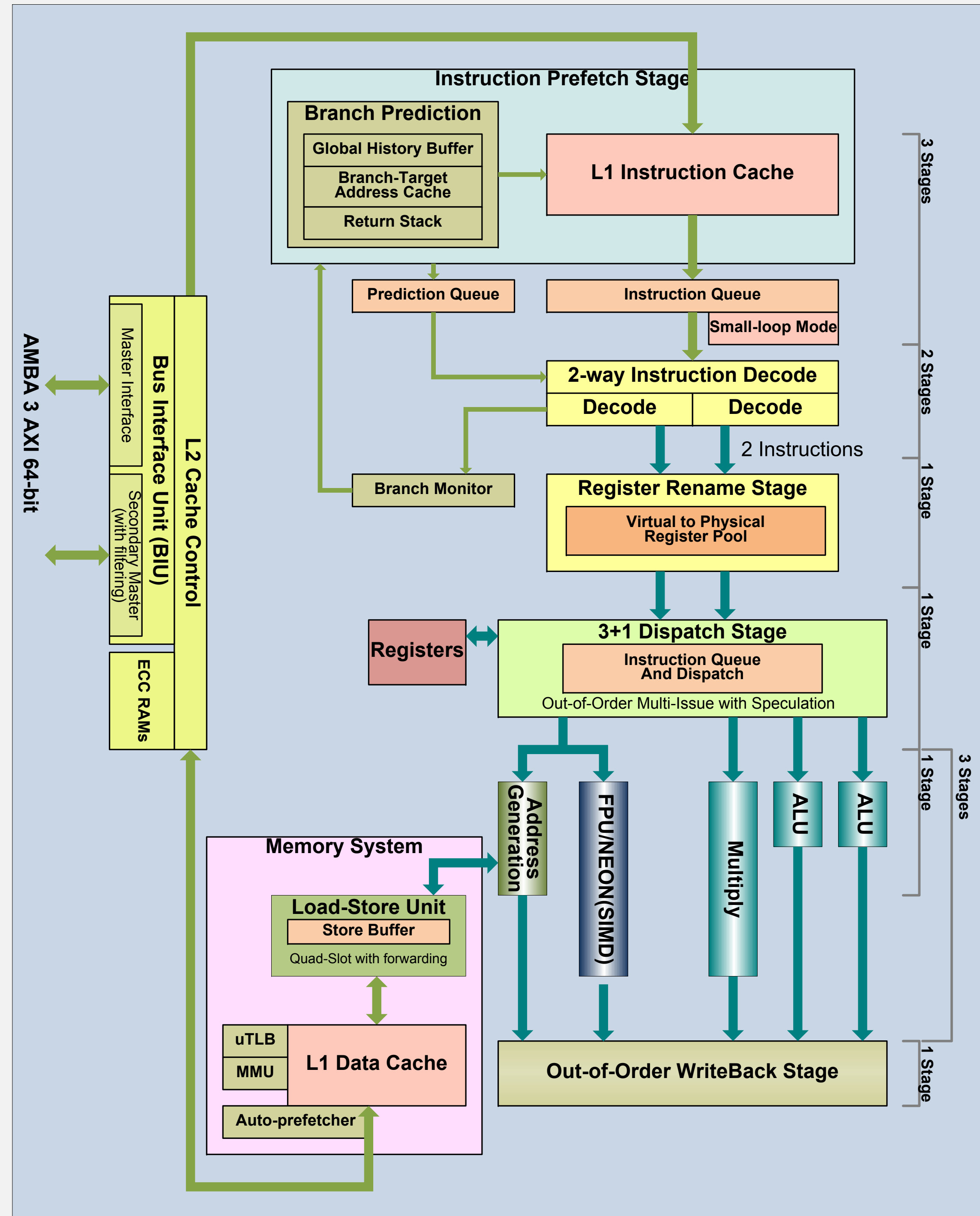
ARM Cortex-A9r4 Core Block Diagram
