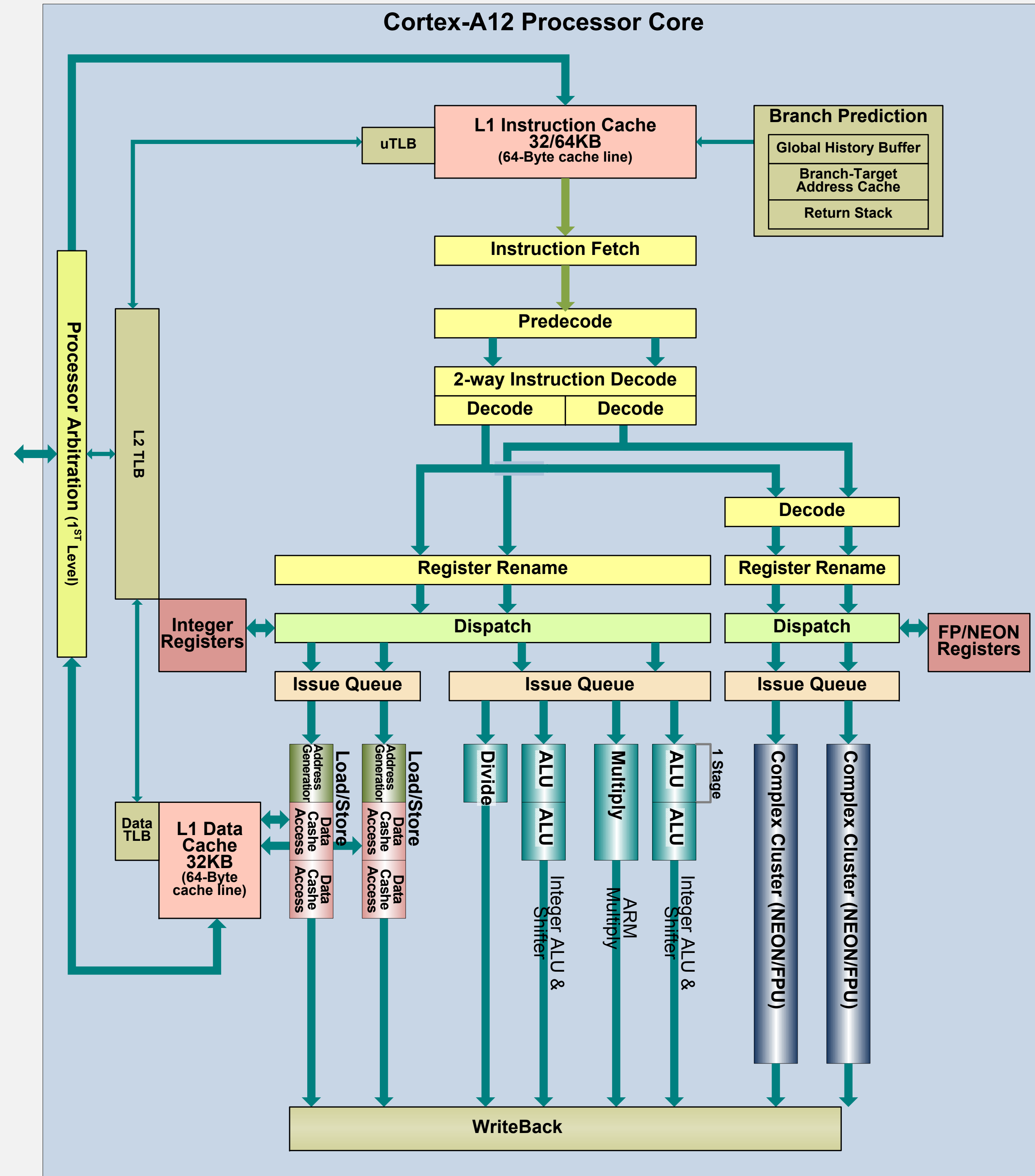
ARM Cortex-A12 Block Diagram
