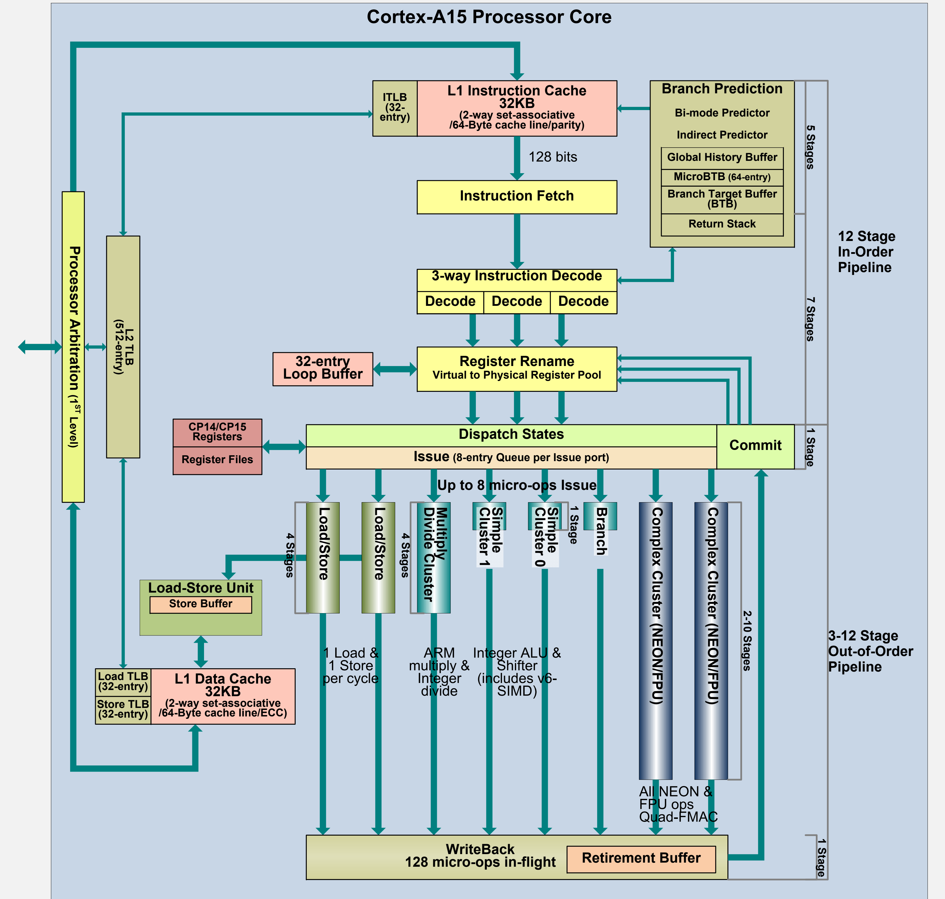
ARM Cortex-A15 Block Diagram
