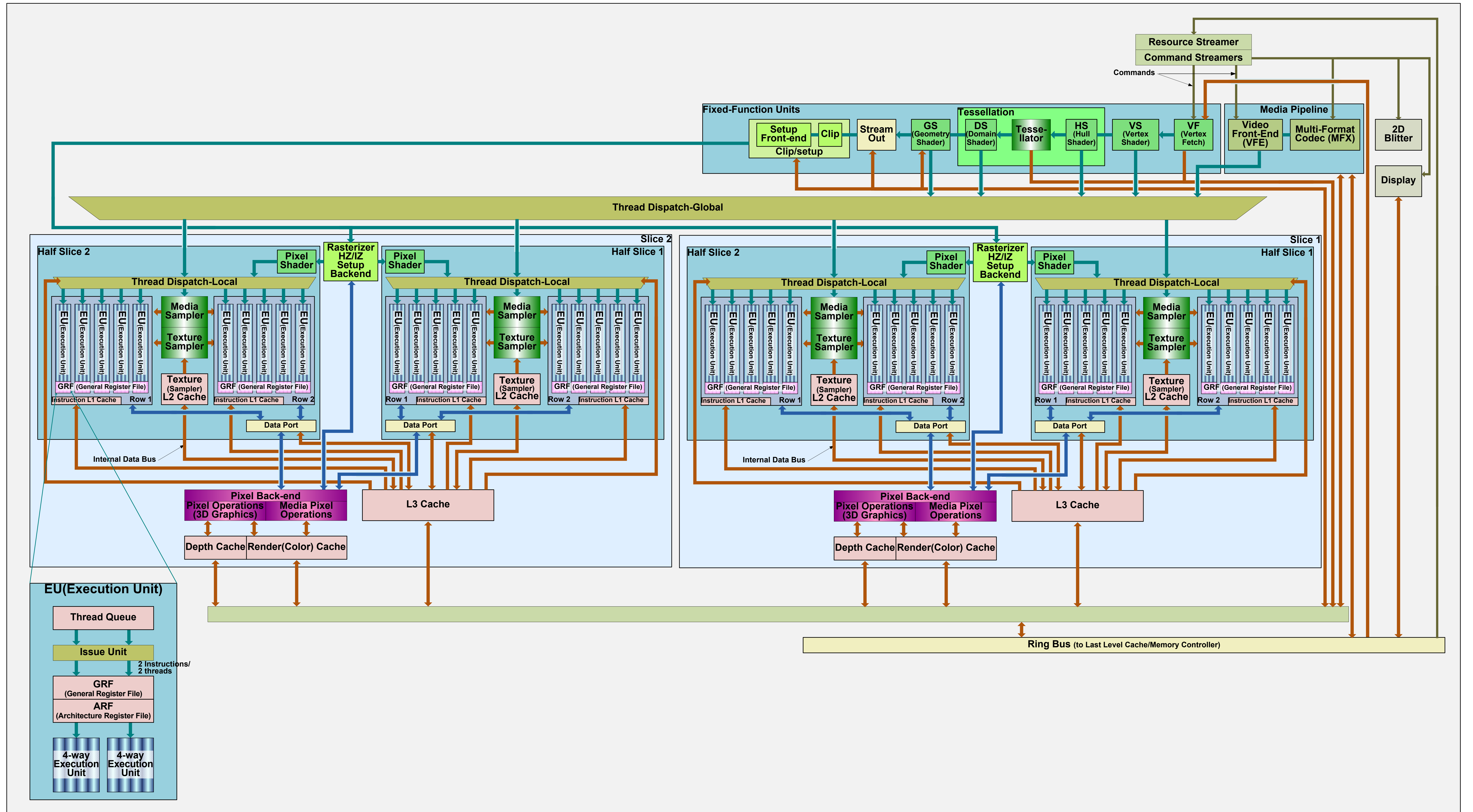
Intel Haswell Graphics Core Diagram (estimated)
