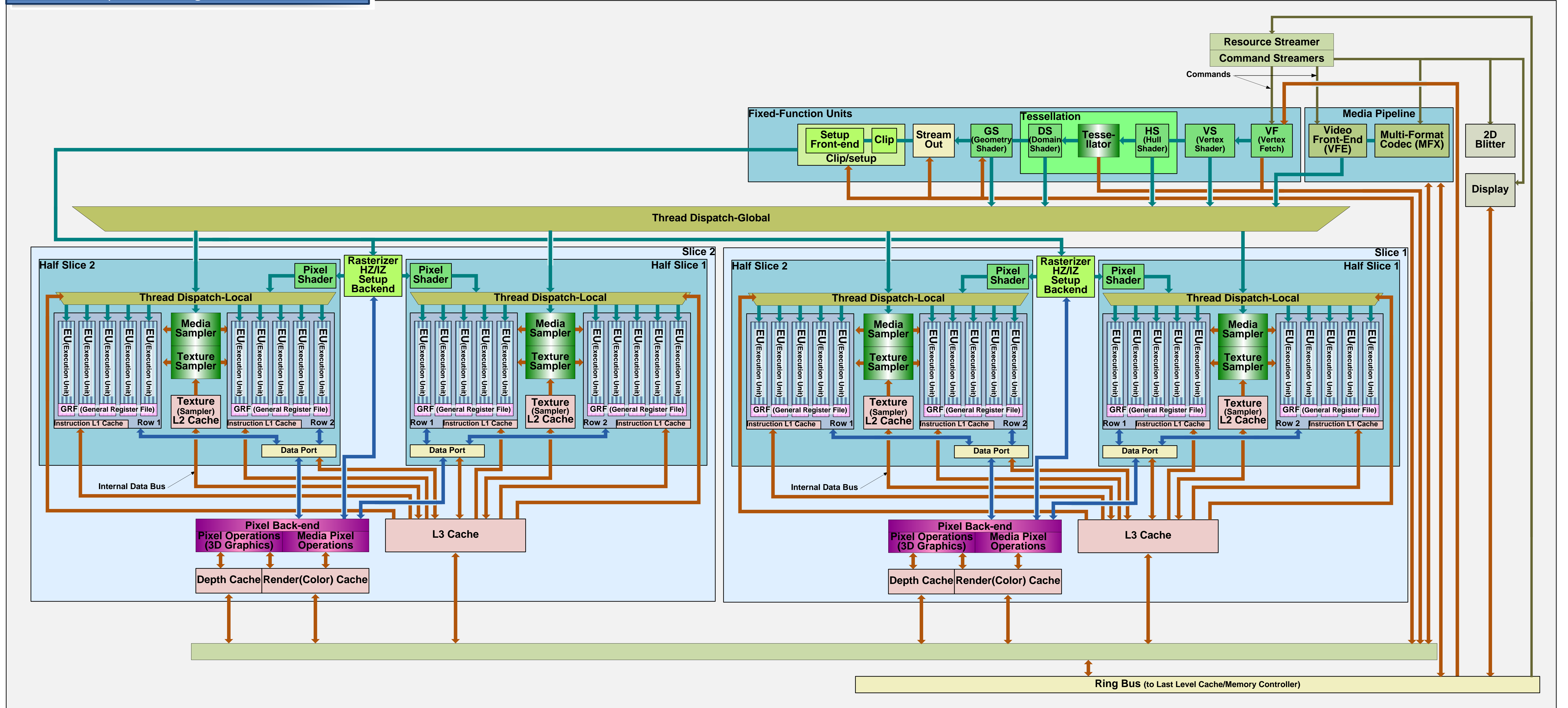
Intel Haswell Graphics Core Diagram (estimated)
