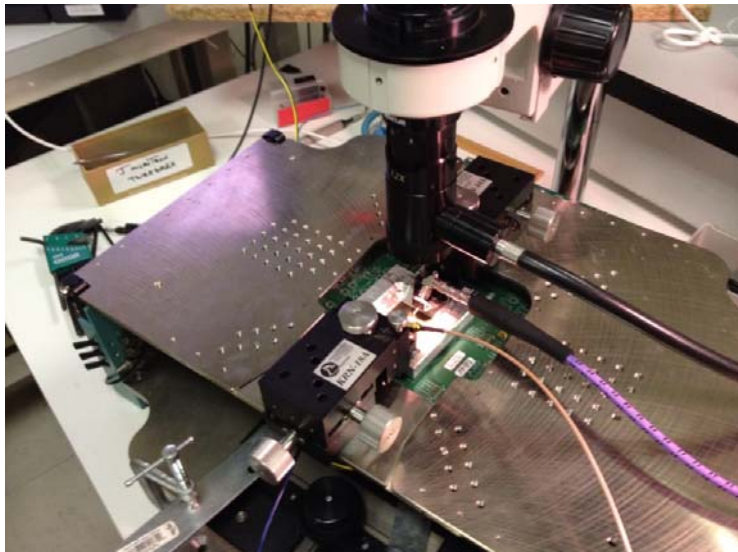
Probe Station
