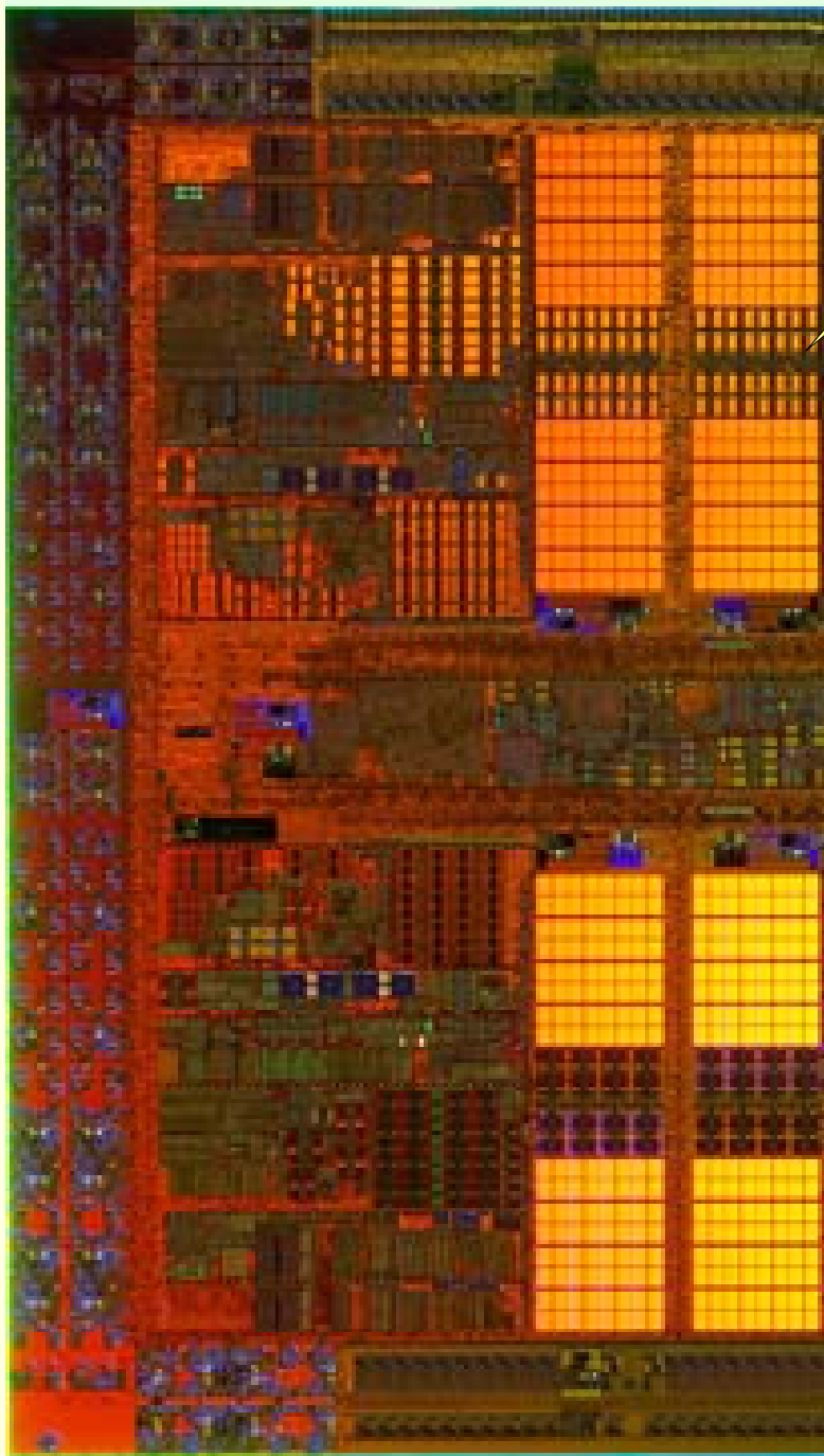
2 Core(1MB L2) without L3
