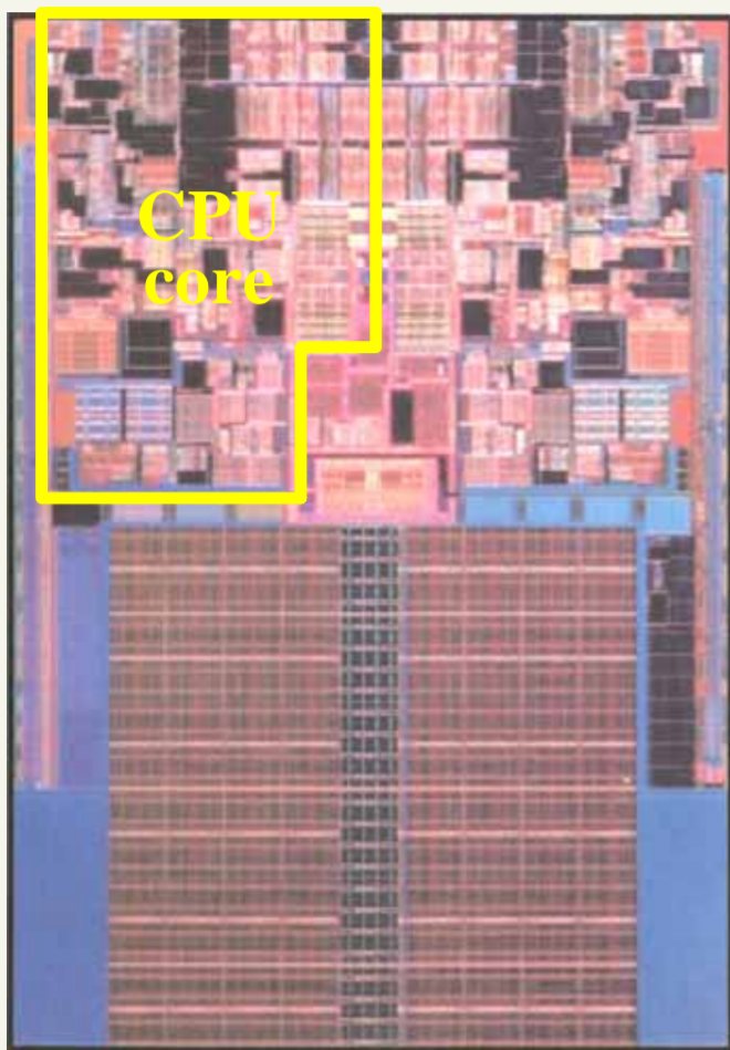
Penryn-6M (Dual-core)
