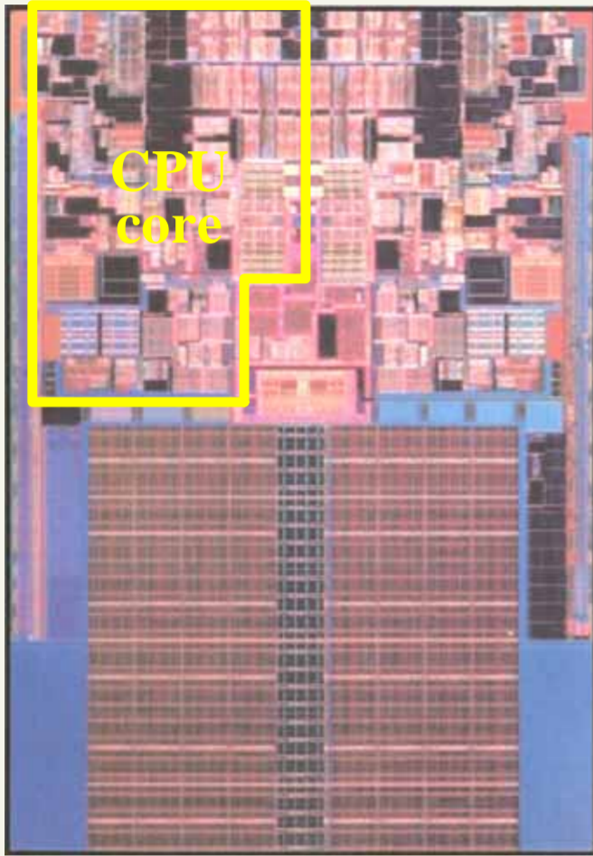
Penryn-6M (Dual-core)
