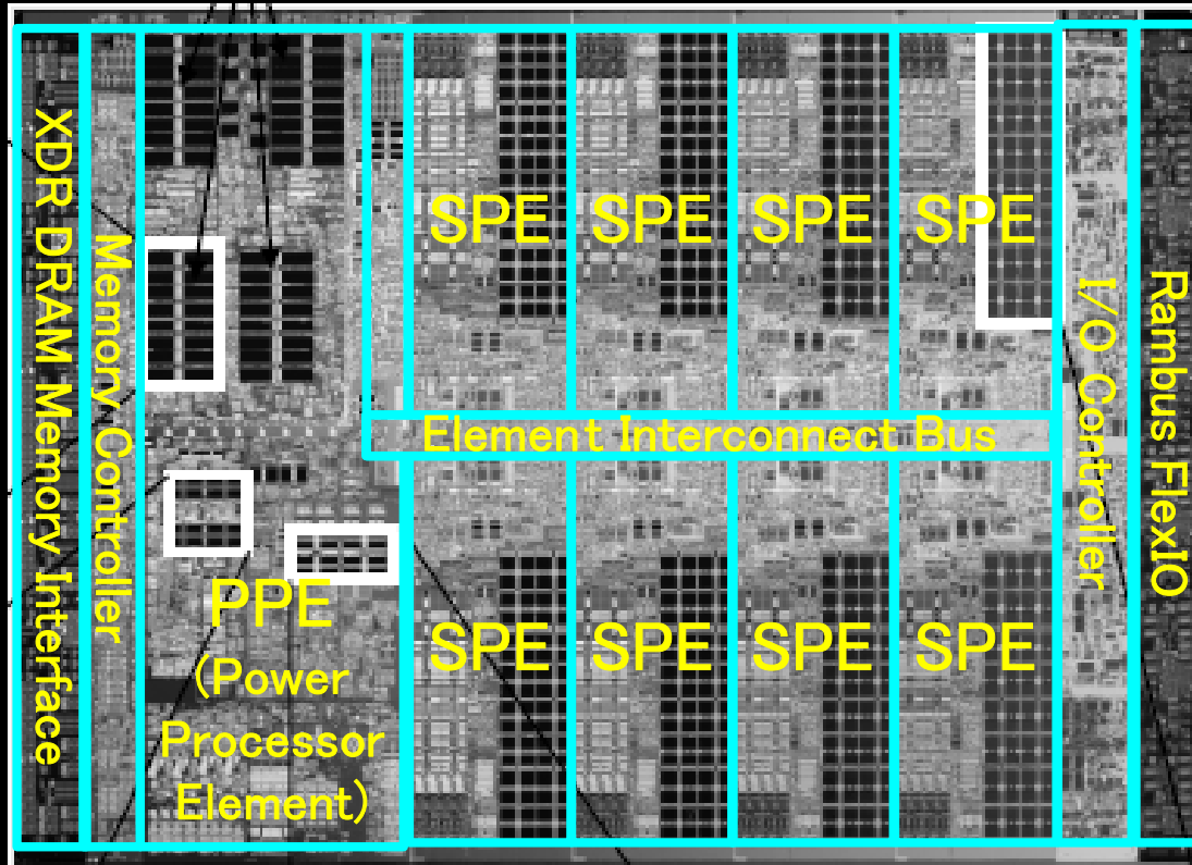
65nm Cell B.E.
