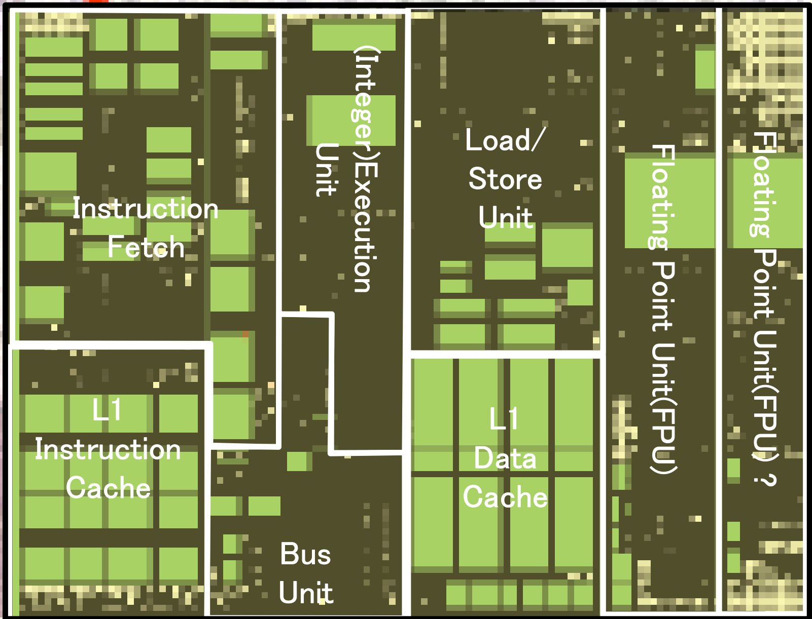
Rev. H? K8 CPU core (SPF May '06)
