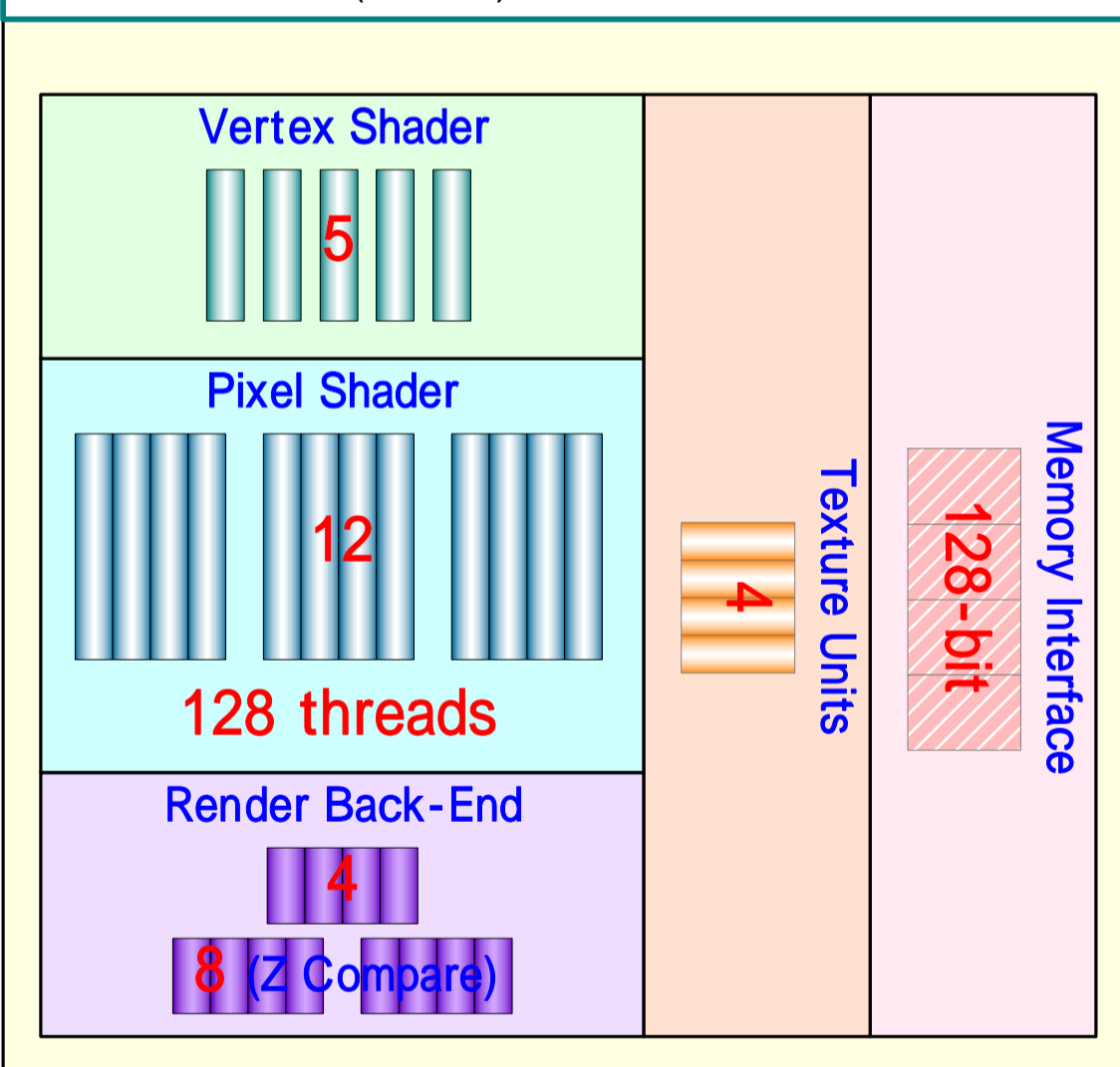
RADEON X1600 (RV530)
